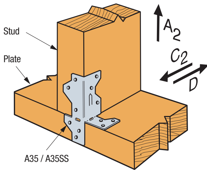
SIMPSON Strong-Tie® A35/A35SS Stud-to-Plate Installation
